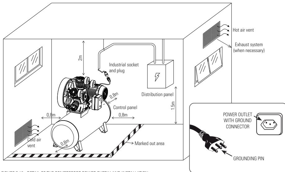
FIGURE 7.10 - DETAIL OF THE COMPRESSOR POWER SUPPLY AND INSTALLATION FROM THE DISTRIBUTION PANEL
