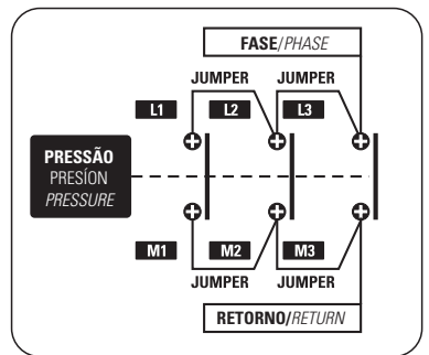
TRIFÁSICO THREE-PHASE
