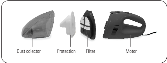
FIGURA 7.1 - MODEL AP 60
